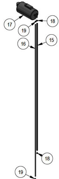
067-0020-01 ZT/Mav EPA Cannister Assy
