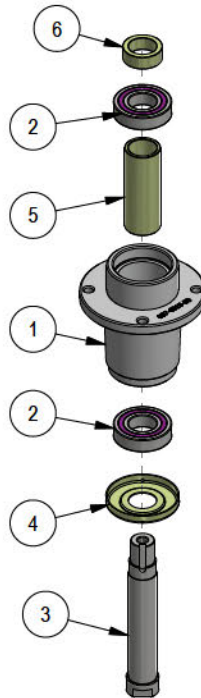
037-6015-50 Spindle Assembly
