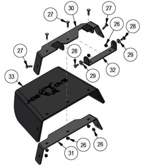
210-6025-01 2026 5in Sloped Deck Rubber Chute Assembly
