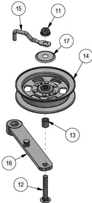
039-6945-27 2027 Maverick HD & Down Deck Idler Assembly
