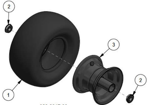
022-2017-00 13x6.5-6 Black Tire and Wheel Assembly
