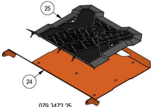
079-3472-25 2025 ZT/Mav/HD Floorboard Assembly
