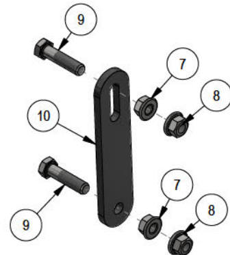
039-2127-17 Deck Hanger Assembly
