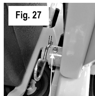
Deck Lift Lever Pivot Grease Fitting
