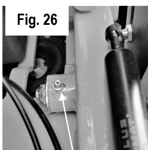
Left Actuator Bar Grease Fitting
