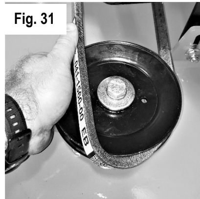
Roll Belt On and Off of Left-hand Spindle Pulley
