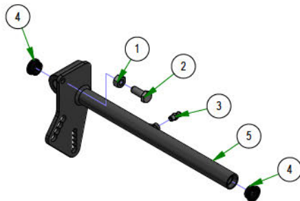
031-0053-21 2021 Maverick Drive Arm Actuator RH Assembly
