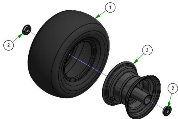
022-2017-00 13x6.5-6 Black Tire and Wheel Assembly
