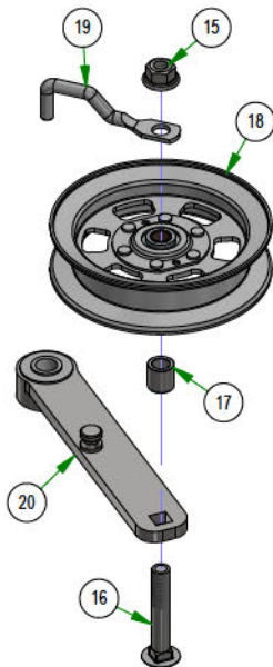
039-6945-26 Marec HD & Down Deck Idler Assembly
