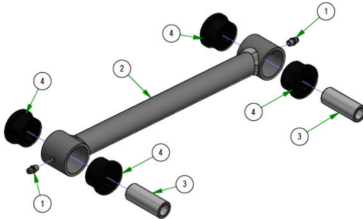
028-0004-22 Hybrid Tumbuckle/Deck Locator
