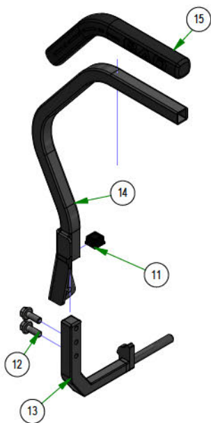
031-9045-00 Small Mower Square Drive Arm RH Assembly
