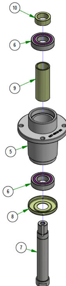
037-6015-50 Spindle Assembly
