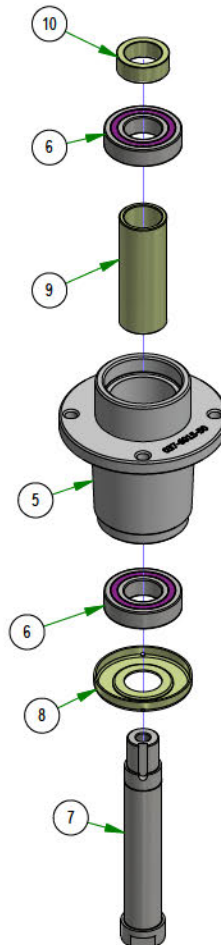
037-6015-50 Spindle Assembly
