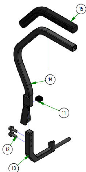
031-9045-00 Small Mower Square Drive Arm RH Assembly
