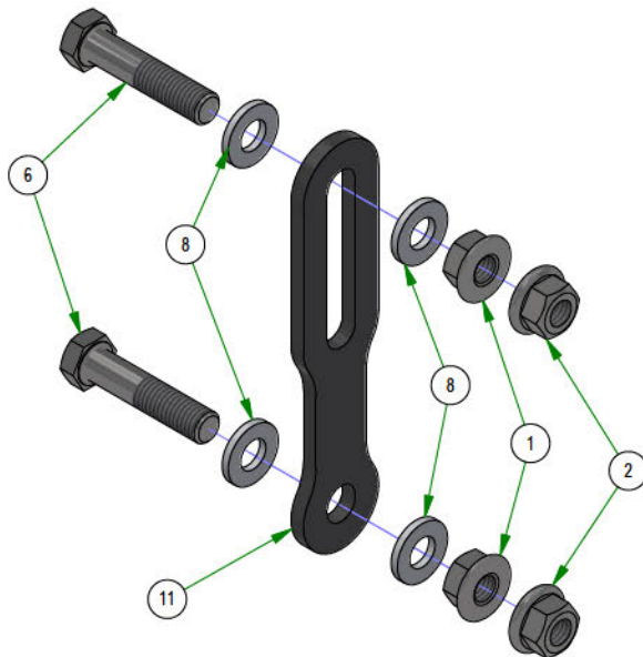
039-2125-17 DECK HANGER
