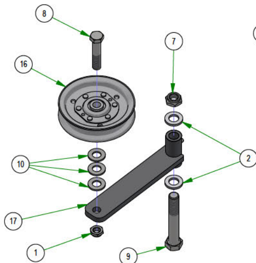
039-0031-19 REAR IDLER PULLEY ASSEMBLY
