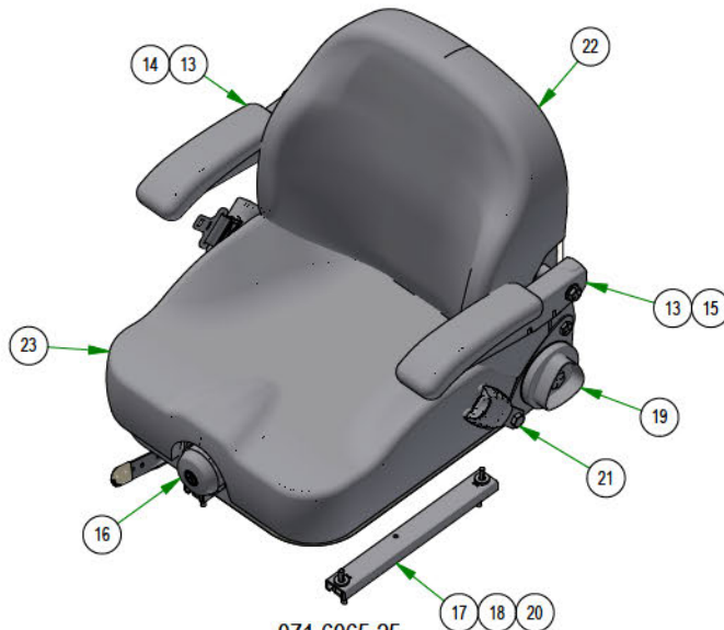
071-6065-25 SEAT ASSEMBLY
