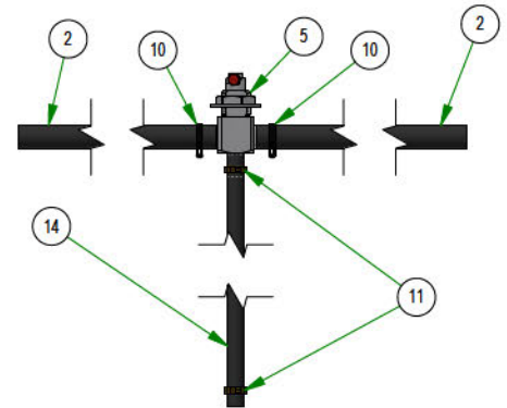
051-2019-33 FUEL LINE ASSEMBLY KOHLER VANGUARD FX1000 EFI
