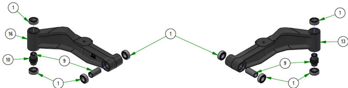
250-0033-54 RH FRONT SUSPENSION ARM 54" DECK
