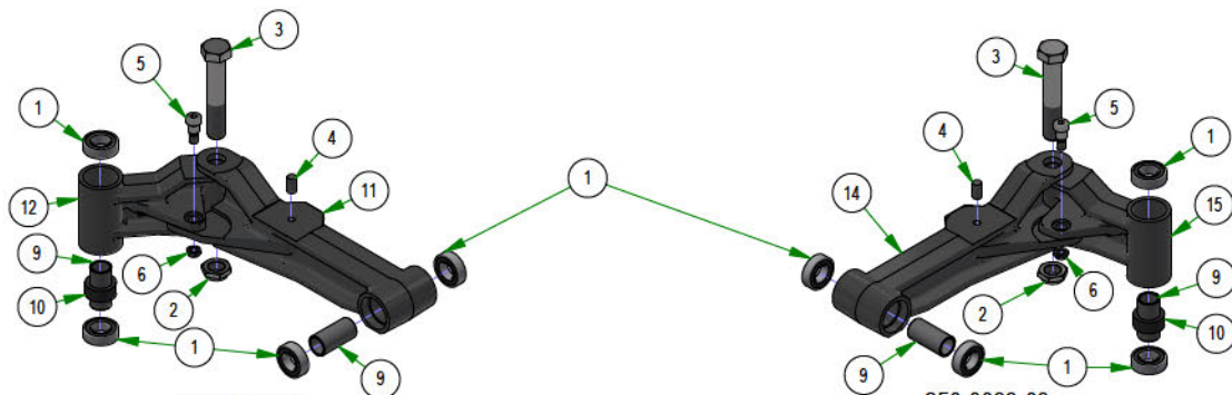
250-0032-03 RH FRONT SUSPENSION ARM 61" & 72" DECK
