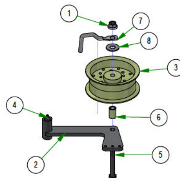
039-6952-23 SD DECK IDLER ASSEMBLY
