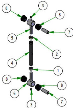
048-6000-00 2018 Maverick Turnbuckle (Top Link)
