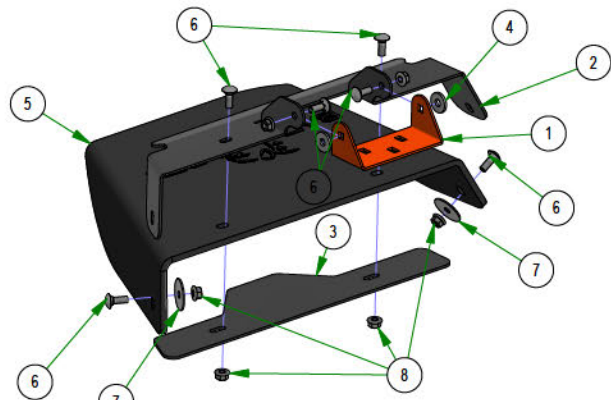
210-6015-98 Discharge Assembly
