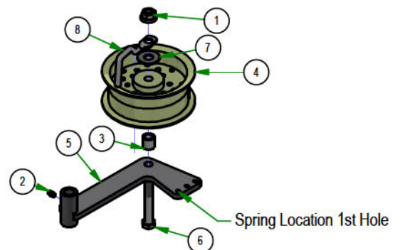
039-6952-98 36 DECK IDLER ASSEMBLY
