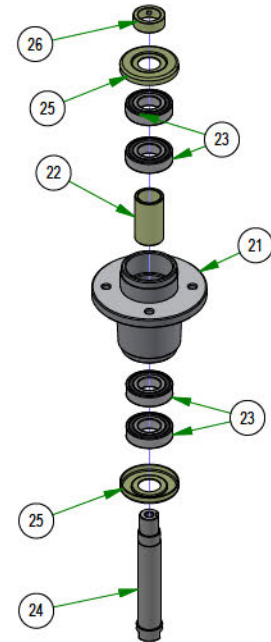
037-4000-00 DECK SPINDLE ASSEMBLY
