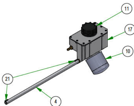
067-8053-18 LH HYDRO TANK ASSEMBLY
