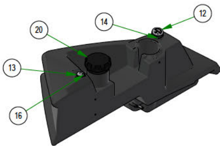
067-9960-50 LEFT FUEL TANK ASSEMBLY
