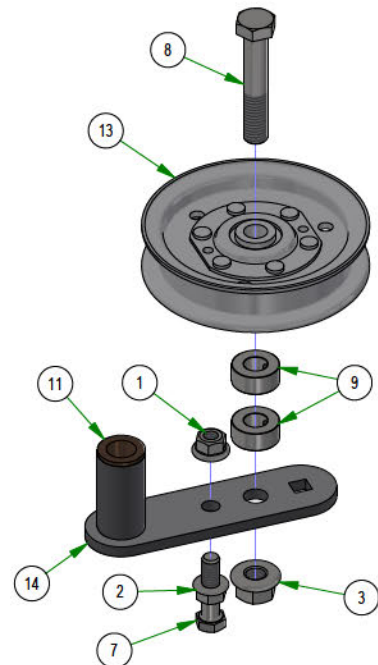
039-6950-95 LEFT PUMP IDLER
