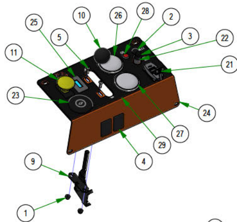
079-3480-22 CONTROL PANEL
