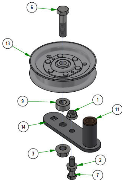
039-6950-94 RIGHT PUMP IDLER
