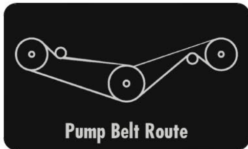
091-4032-00 2019 Renegade Pump Belt Route Decal
