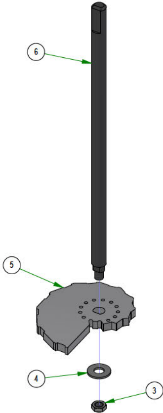
028-0015-19 DECK HEIGHT CAM ASSEMBLY
