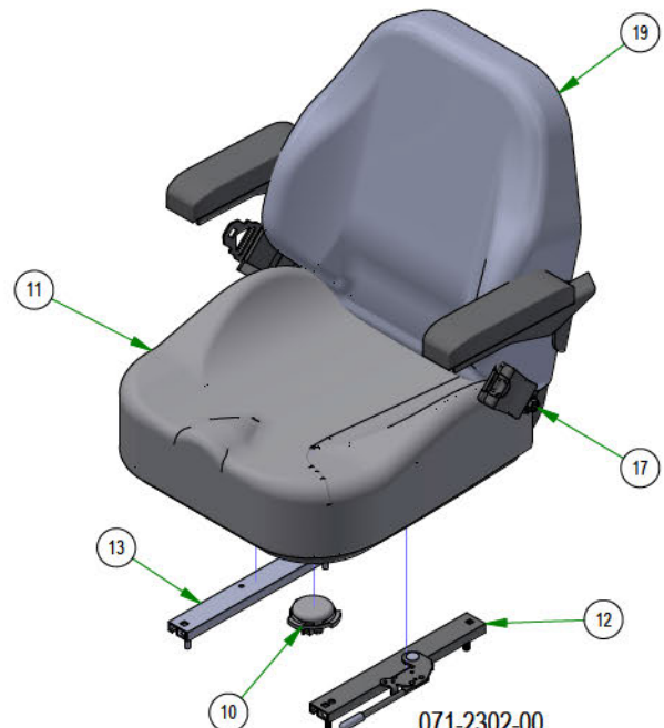
071-2302-00 SEAT ASSEMBLY
