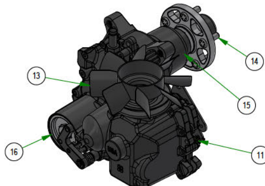
050-1000-00 & 050-1050-00 REBEL 4400 TRANSAXLE PARTS
