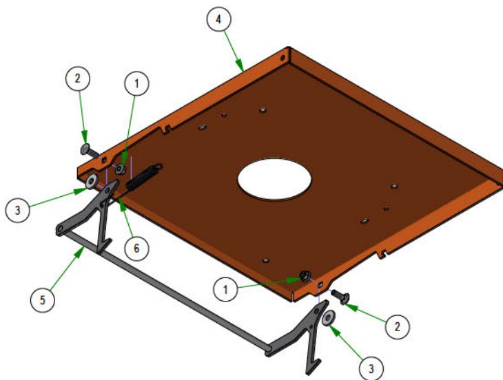
026-2019-21 SEAT PLATE ASSEMBLY
