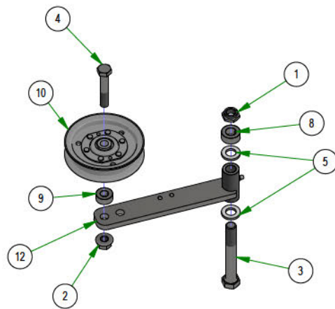
039-6945-03 TRANSAXLE IDLER ASSEMBLY
