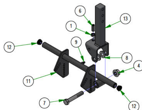
031-0031-24 LH DRIVE PIVOT ASSEMBLY
