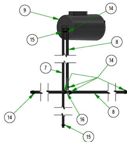
067-0020-19 EPA CANISTER ASSEMBLY
