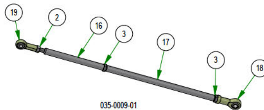
035-0009-01 PUSH ROD ASSEMBLY
