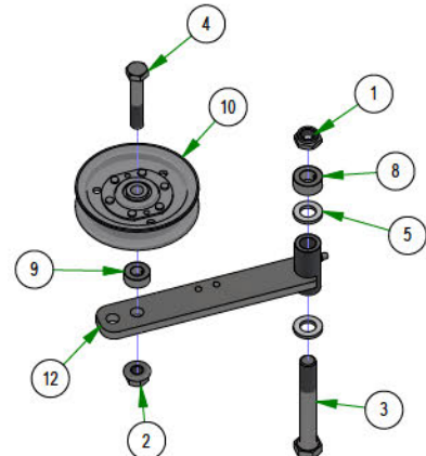
039-6945-RX REBEL X TRANSAXLE IDLER ASSEMBLY
