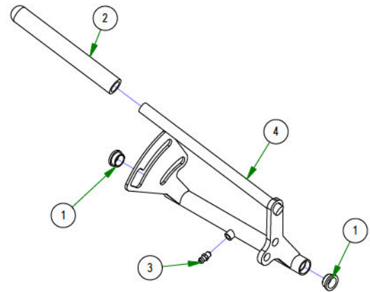
031-0042-00 2020 Walk-Behind Control Lever Assembly - Left
