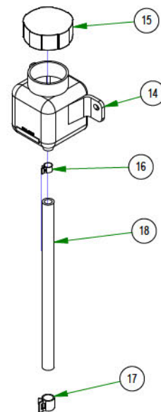
067-8090-04 Walk Behind Hydro Tank Assembly
