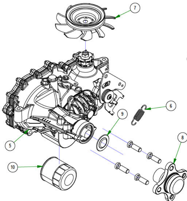
050-0003-02 Walk Behind Transaxle Left 3100
