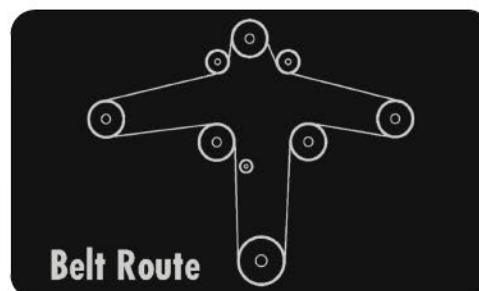
091-3309-00 Deck Belt Route Decal
