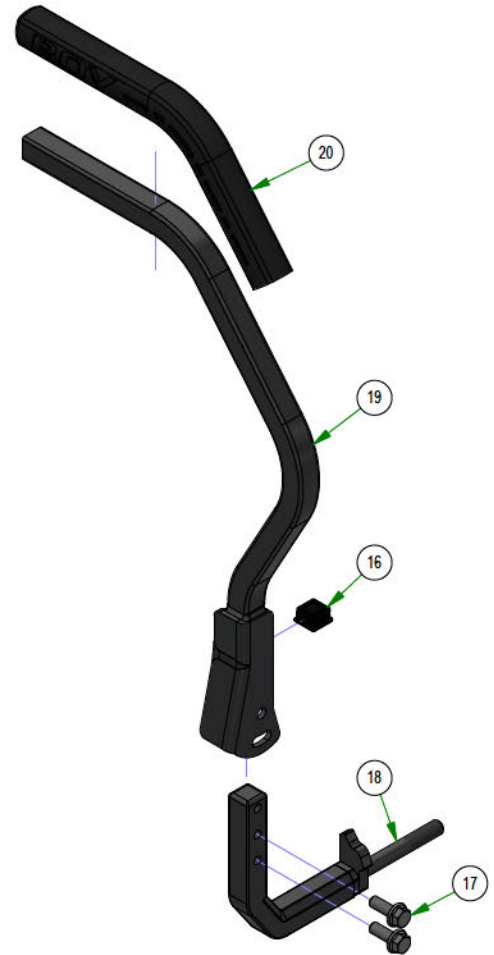
031-9046-00 Small Mower Square Drive Arm LH Assembly
