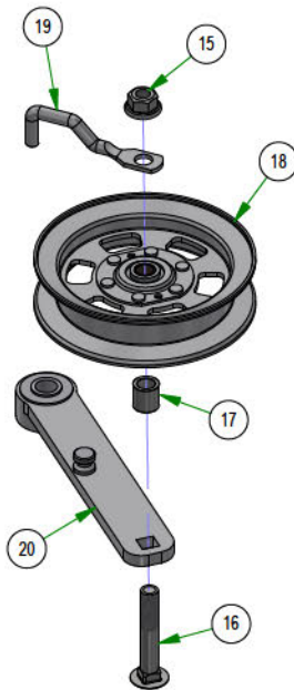
039-6945-26 Marenick HD & Down Deck Idler Assembly
