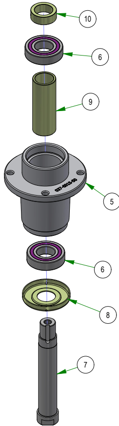
037-6015-50 Spindle Assembly
