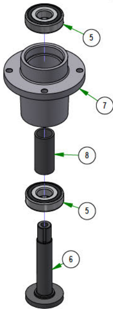
037-2000-00 Spindle Assembly-MZ
