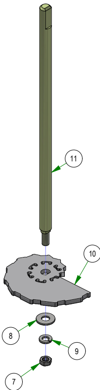
028-0070-17 ZT Deck Height Bar Assembly
