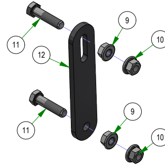
039-2127-17 Deck Hanger Assembly
