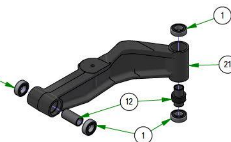
250-0032-54 LH FRONT SUSPENSION ARM 54" DECK
