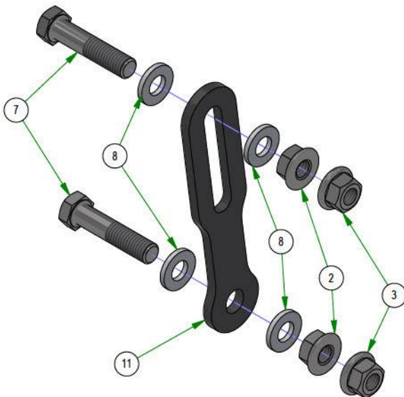
039-2125-17 DECK HANGER
