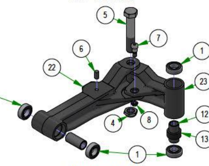
250-0033-03 LH FRONT SUSPENSION ARM 61" & 72" DECK
