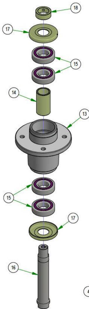
037-4000-00 SPINDLE ASSEMBLY
