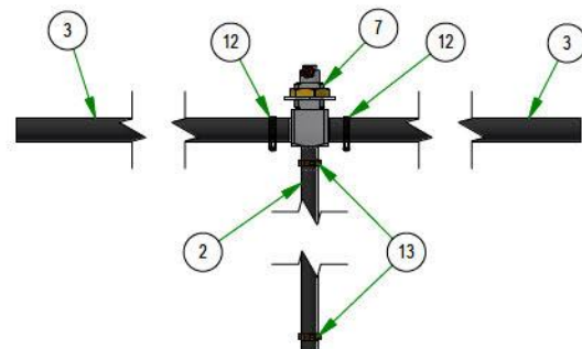
051-2019-33 FUEL LINE ASSEMBLY KOHLER VANGUARD FX1000 EFI
