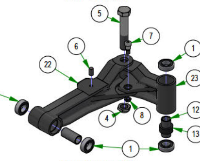
250-0033-03 LH FRONT SUSPENSION ARM 61" & 72" DECK
