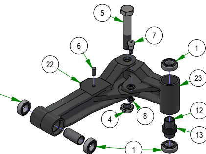
250-0033-03 LH FRONT SUSPENSION ARM 61" & 72" DECK
