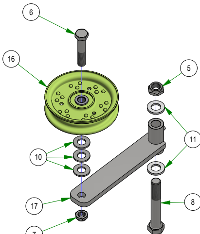
039-0031-19 REAR IDLER PULLEY ASSEMBLY
