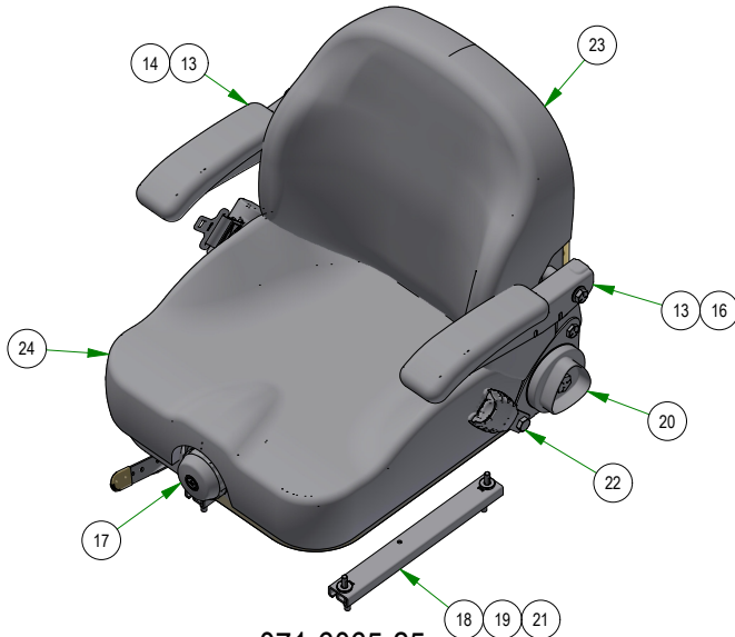
071-6065-25 SEAT ASSEMBLY
