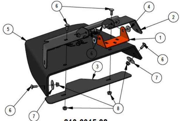
210-6015-98 Discharge Assembly
