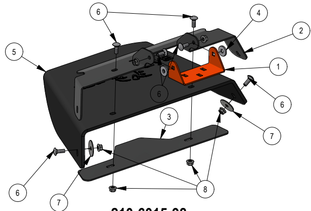
210-6015-98 Discharge Assembly
