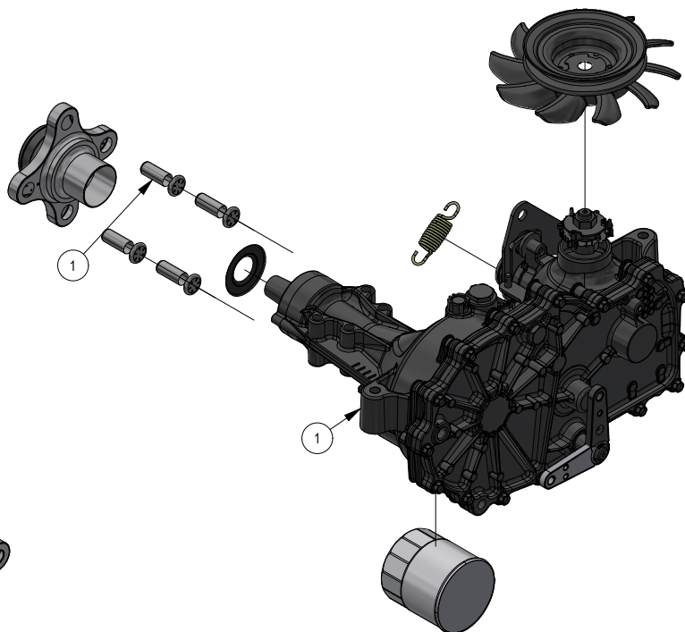
050-0004-02 Walk Behind Transaxle Right 3100
