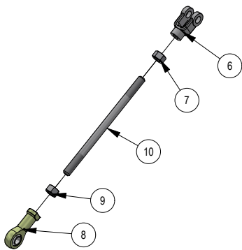
035-0002-98 Walk Speed Control Linkage
