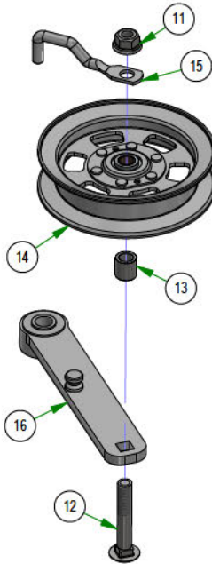
039-6945-26 Marec HD & Down Deck Idler Assembly
