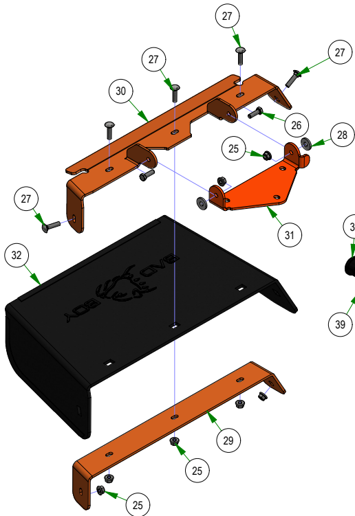
210-6005-98 Discharge Chute Assembly 54" & 60" Decks
