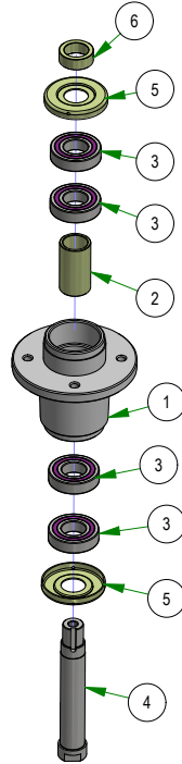
037-4000-00 Outlaw Spindle Assembly
