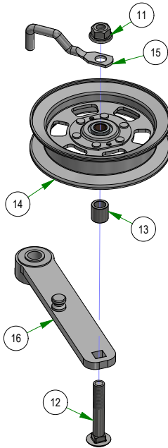
039-6945-26 Maverick HD & Down Deck Idler Assembly
