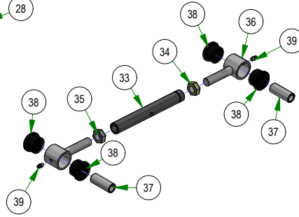
048-6000-00 2018 Maverick Turnbuckle (Top Link)
