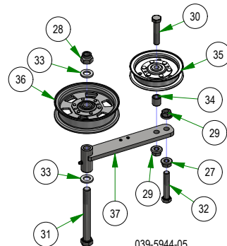
039-5944-05 Maverick Pump Idler
