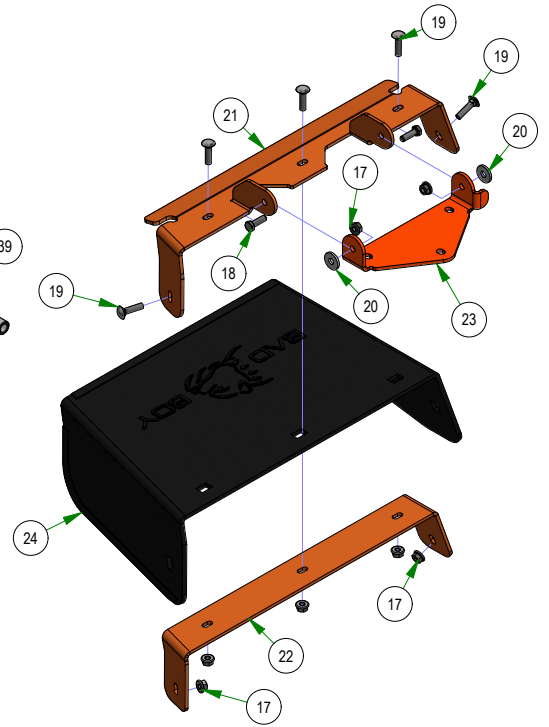
210-6005-48 ZT Chute Assembly 42" & 48" Decks
