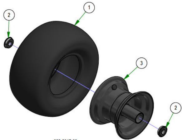
022-2017-00 13x6.5-6 Black Tire and Wheel Assembly
