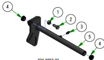
031-0053-21 2021 Maverick Drive Arm Actuator RH Assembly
