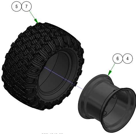
022-4040-00 23x9-12 Reaper Turf Tire & Wheel Assembly & 022-4200-00 23x11-12 Reaper Turf Assembly
