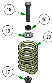
034-8045-03 Seat Spring Assembly
