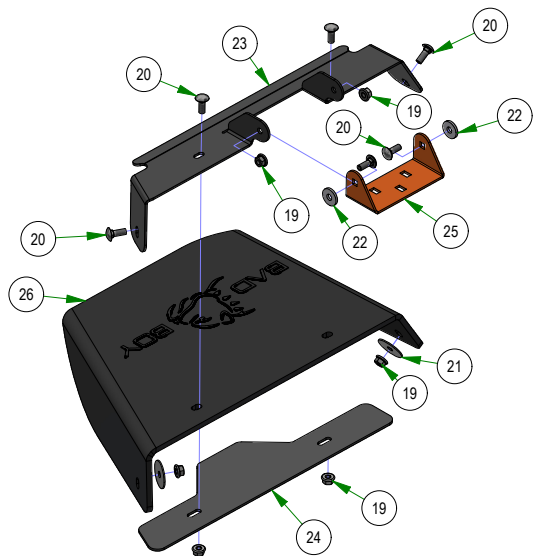
210-6015-98 MZ Discharge Chute Assembly
