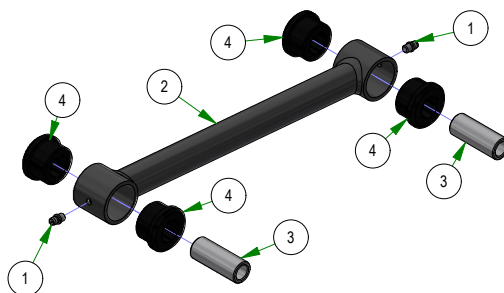
028-0004-22 Hybrid Turnbuckle/Deck Locator
