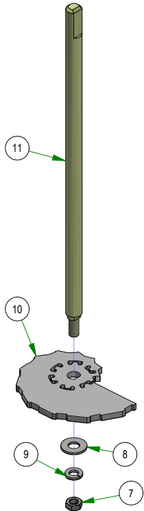
028-0070-17 ZT Deck Height Bar Assembly
