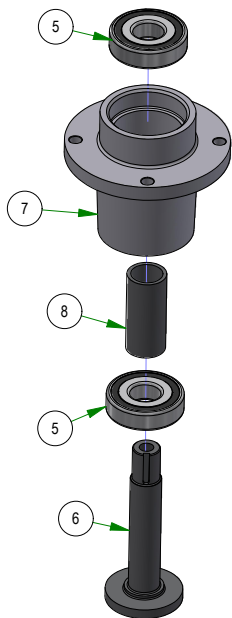
037-2000-00 Spindle Assembly-MZ
