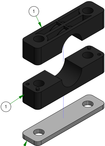
017-9076-00 Pillow Block Kit
