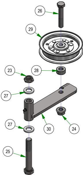
039-5944-01 ZT Pump Idler
