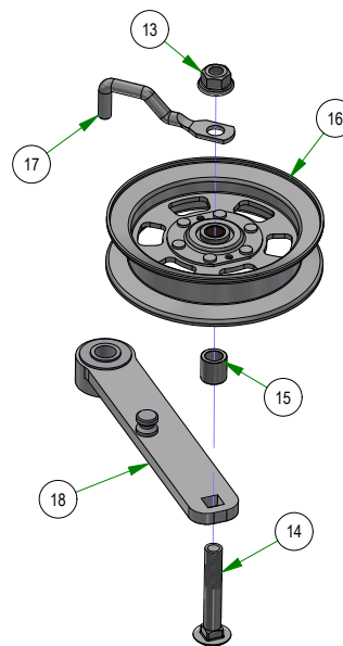
039-6945-26 Maverick HD & Down Deck Idler Assembly
