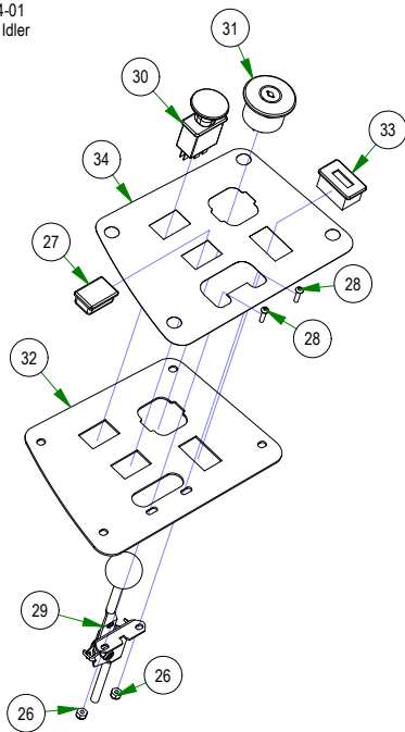
079-3560-23 2023 Control Panel Assembly
