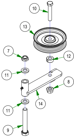
039-5944-01 ZT Pump Idler
