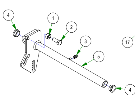
031-0053-21 2021 Maverick Drive Arm Actuator RH Assembly
