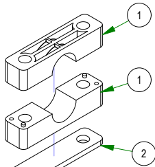
017-9076-00 Pillow Block Kit
