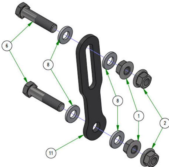
039-2125-17 DECK HANGER
