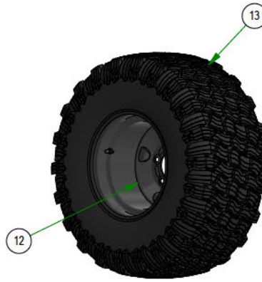
022-4091-00 REAR WHEEL ASSEMBLY 54" DECK
