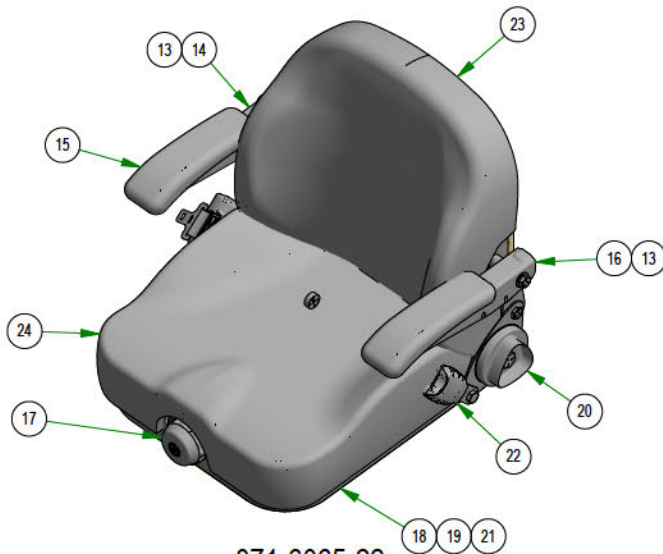
071-6065-22 SEAT ASSEMBLY
