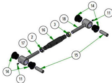
048-8000-00 TURNBUCKLE ASSEMBLY
