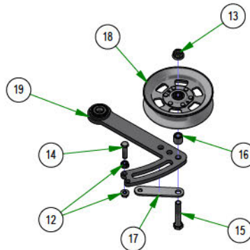
039-6946-17 2019 Renegade Deck Idler
