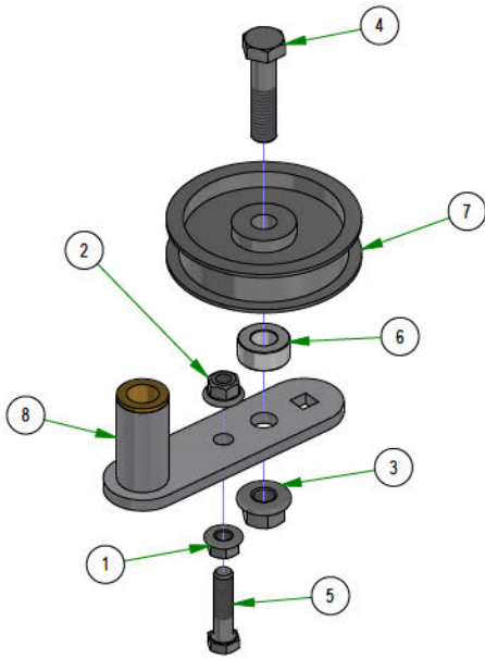
039-6950-98 2019 Renegade Belt Tensioner LH
