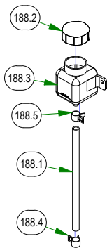
067-8090-03 Hydro Tank Assembly
