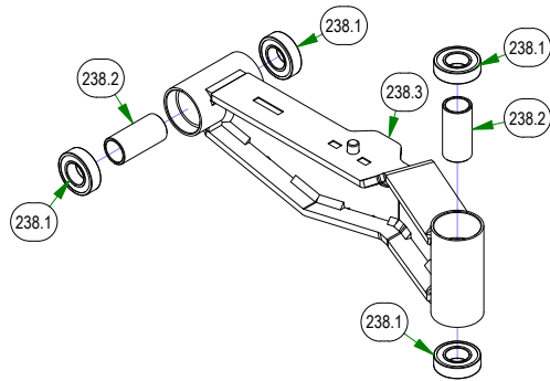
250-2801-21 2021 Maverick LH Front Suspension Arm Assy (48", 54" & 60")
