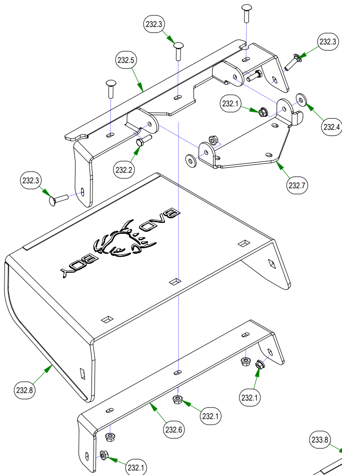
210-6005-48 ZT Chute Assembly
