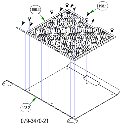
079-3470-21 2021 Maverick Floorboard Assembly
