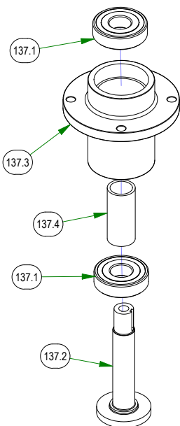
037-2000-00 Spindle Assembly-MZ
