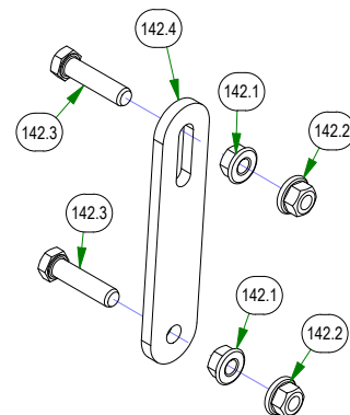
039-2127-17 Deck Hanger Assembly
