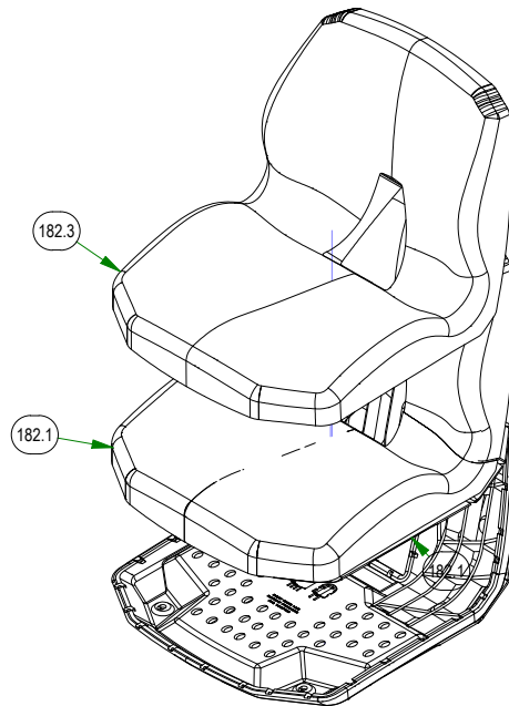
071-1000-22 2022 Magnum Seat
