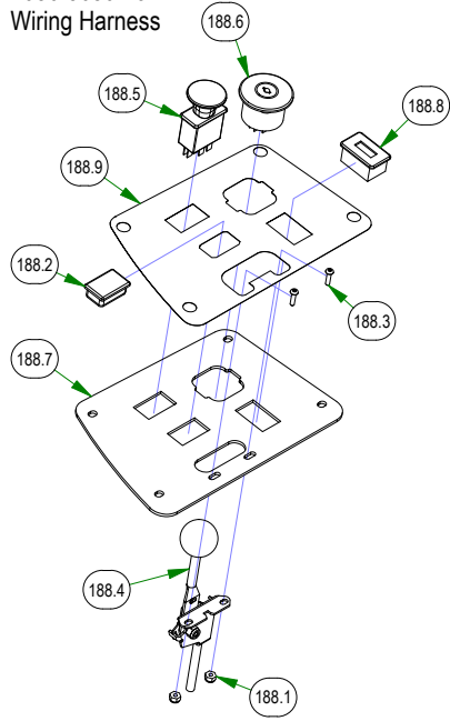
079-3460-19 2019 ZT/Maverick Control Panel Assembly
