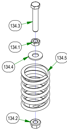
034-8045-03 Seat Spring Assembly
