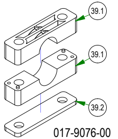
017-9076-00 Pillow Block Kit
