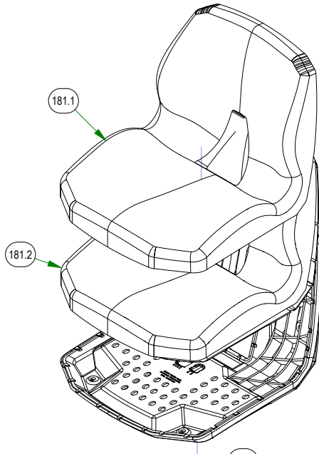
071-1000-00 2019 Magnum Seat/Kohler
