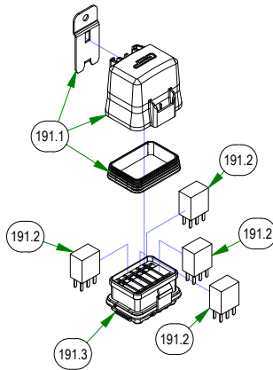
086-3050-19 Wiring Harness
