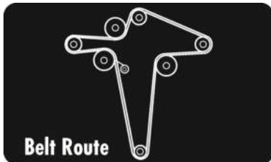
091-0393-00 2017 MZ Magnum 48"/42" Deck Route Decal
