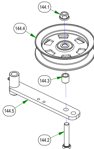
039-6945-18 2017 54"/48" Deck Idler Assembly
