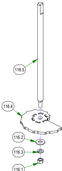
028-0007-17 Deck Height Dial Rod Assembly
