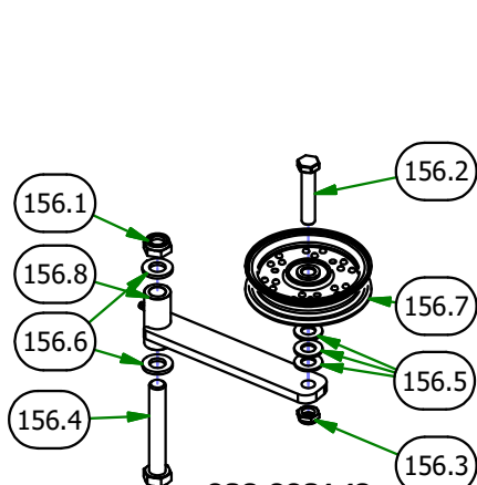
039-0031-19 2019 Rogue Pump Idler Assy
