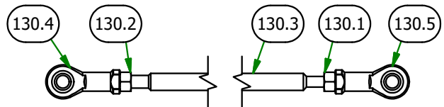
035-0003-00 2019 Rebel Push Rod Assembly
