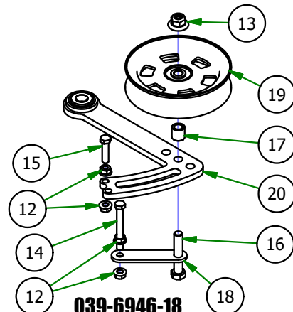
039-6946-18 2019 Rebel Rogue Deck Idler
