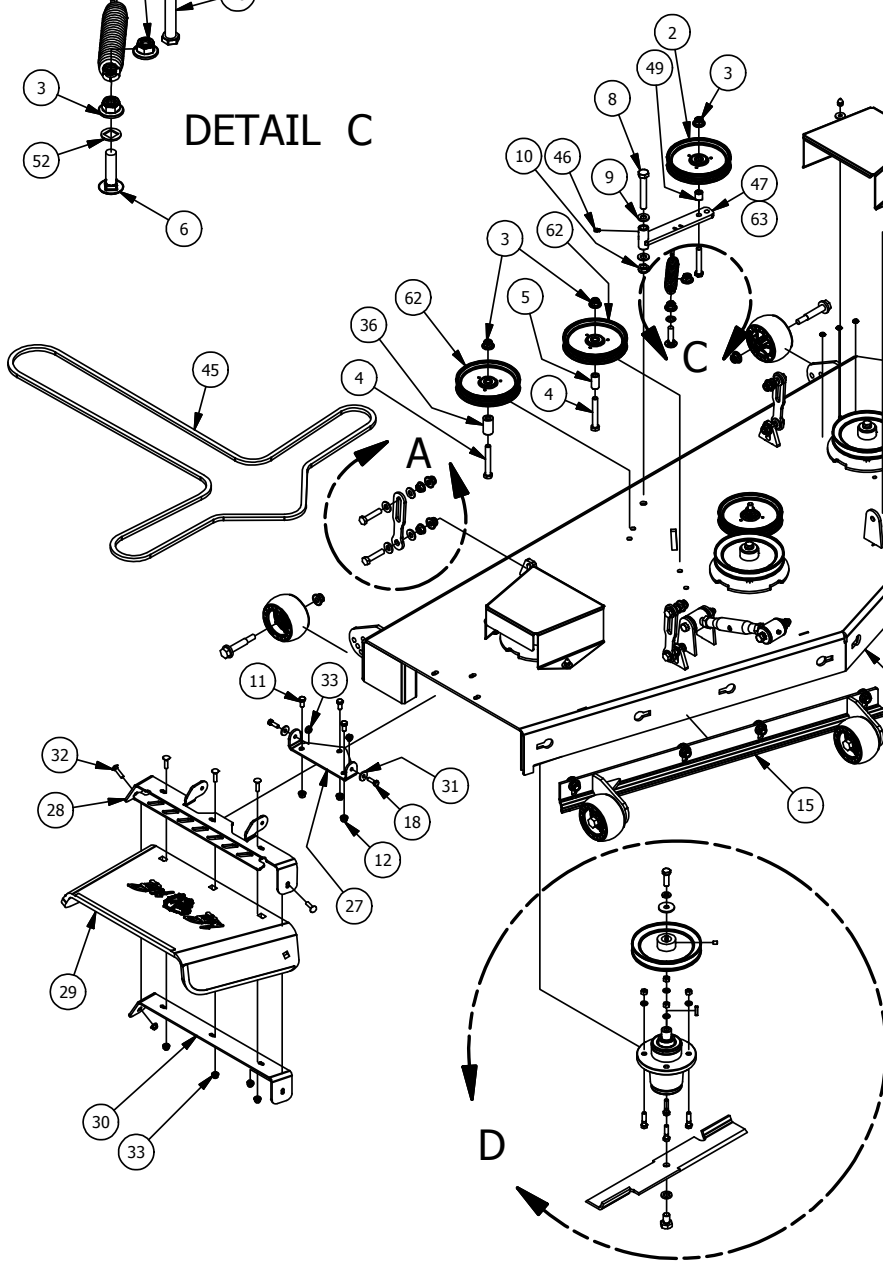
DETAIL D
